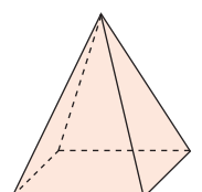
Pyramide
