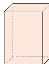
Quader
