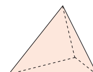
Tetraeder
