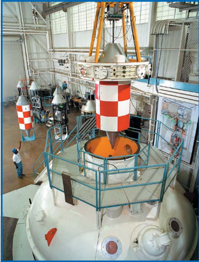
Positioning a drop vehicle on top of the vacuum chamber.
