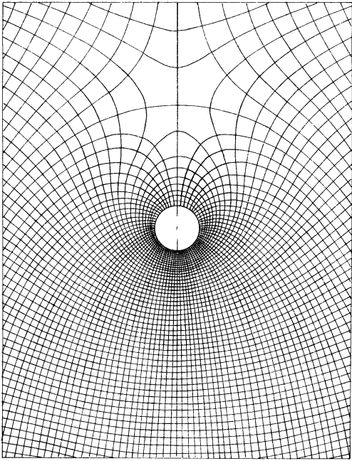
Fig. 1. Diagram of the superposition of the magnetic field of a linear current and a homogeneous magnetic field, in “Electricity and Magnetism”, by Maxwell. All of Maxwell's figures display “lines of force” and “level surfaces”.
