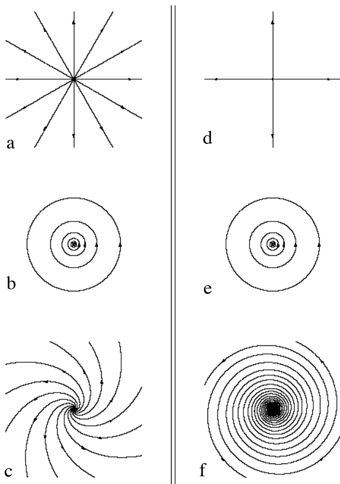
Fig. 2. (a) Electric field of a line charge. (b) Electric field of a thin solenoid with a magnetic flux changing at a constant rate. (c) Superposition of the fields of (a) and (b). (d) Field of a line charge with smaller charge density. (e) the same as (b). (f) Superposition of the fields of (d) and (e). The field line density suggests a higher magnitude of the field strength than the field actually has.
