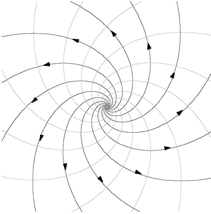
Fig. 3. The same field as that of Fig. 2c. In addition to the field lines the orthogonal lines are represented. Both ensembles of lines end within the small circle in the center of the figure. Thus, this circle must contain the flux sources as well as the circulation sources of the field.
