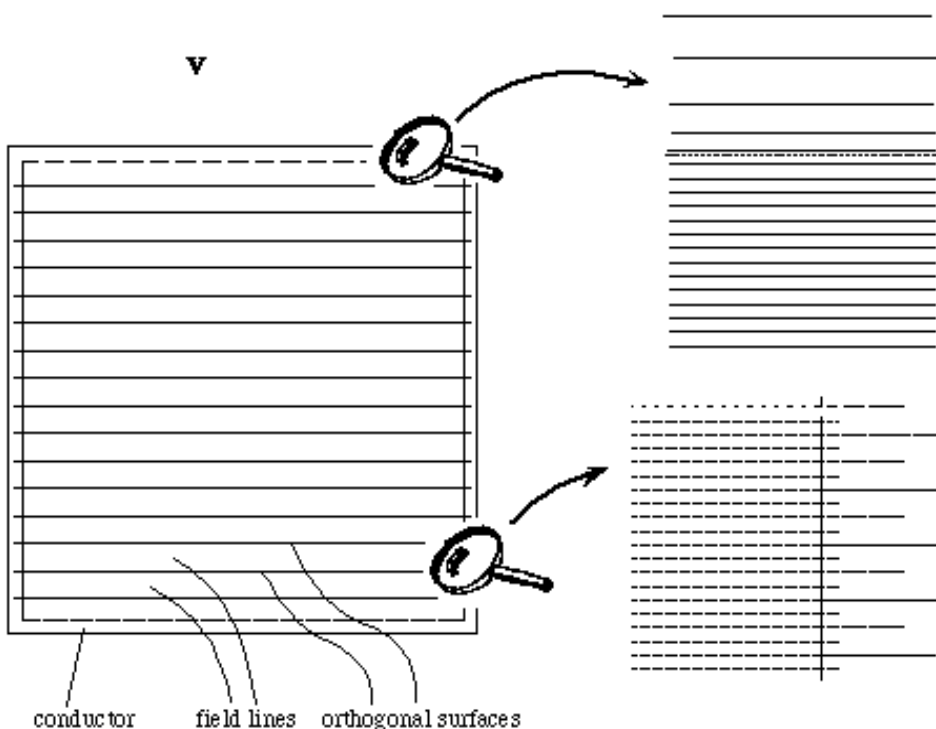
Fig. 5. Field lines and orthogonal surfaces of the rectangular field. It is seen that the flux sources are located on the lateral parts of the sheet (parallel to the direction of the movement) and the circulation sources on the transverse parts (perpendicular to the movement). The enlargements of a section of the transverse part and of a section of the parallel part of the conductor show that the field lines end within the bulk of the parallel parts and the orthogonal lines end within the bulk of the transverse parts.
